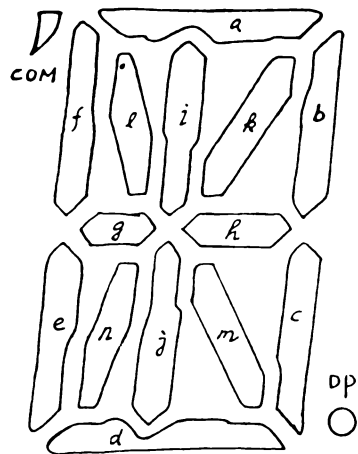
Fig. 8-12 Segment Pattern
