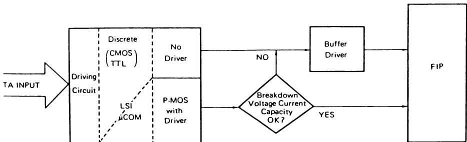
Fig. 8-8 Determination of Necessity of Buffer-Driver
