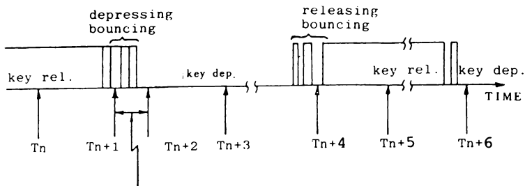
Fig. 8-11 The Time Response of Keyboard Scanning
